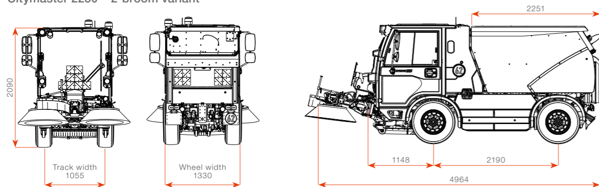
Citymaster 2250 – 2-broom variant
